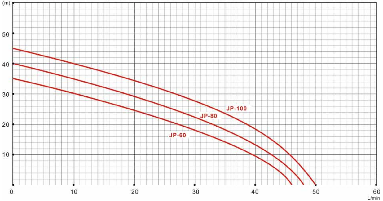
H PERFORMANCE CHART AT n=2850 r/ min
